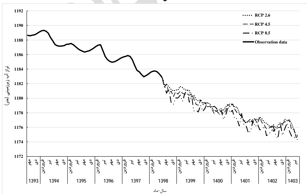
ب - EC-ERATH
