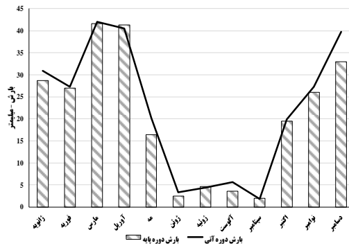
RCP 4.5
