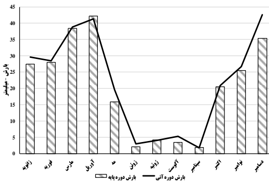
RCP 8.5
