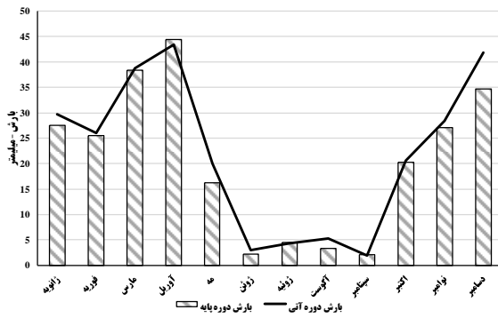
RCP 4.5
